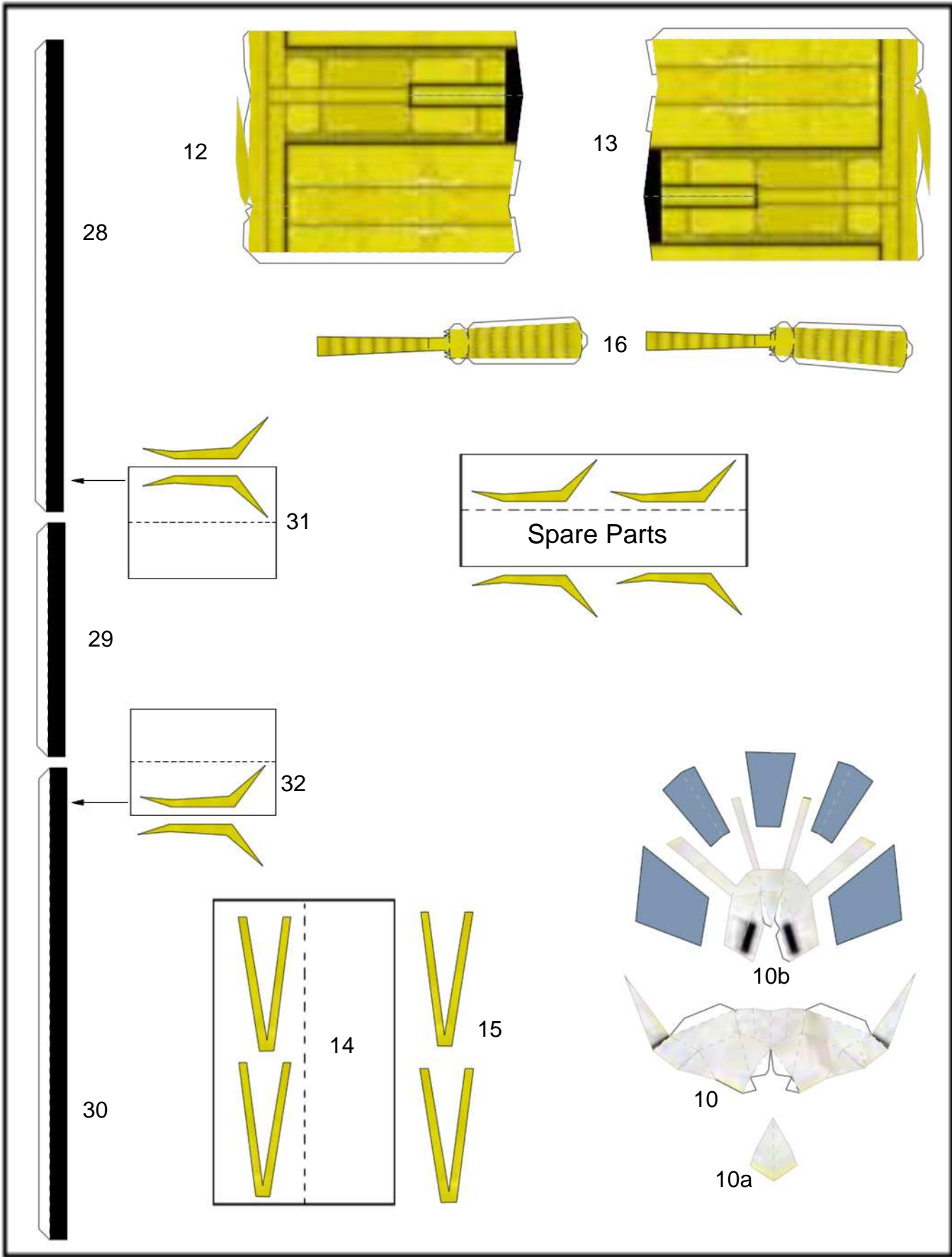
Airtractor AT-502B Paper Model, Copyright 2006 by Steve Bondy, Scale 1/48
